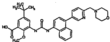
5-tert-Butyl-2-methoxy-3-{3-[4-(6-morpholin-4-ylmethyl-pyridin-3-yl)-naphthalen-1-yl]-ureido}-benzoic acid;
